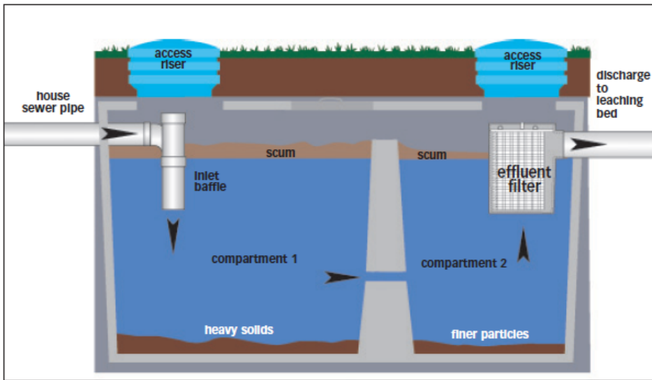
Figure 12: Parts of a septic system
